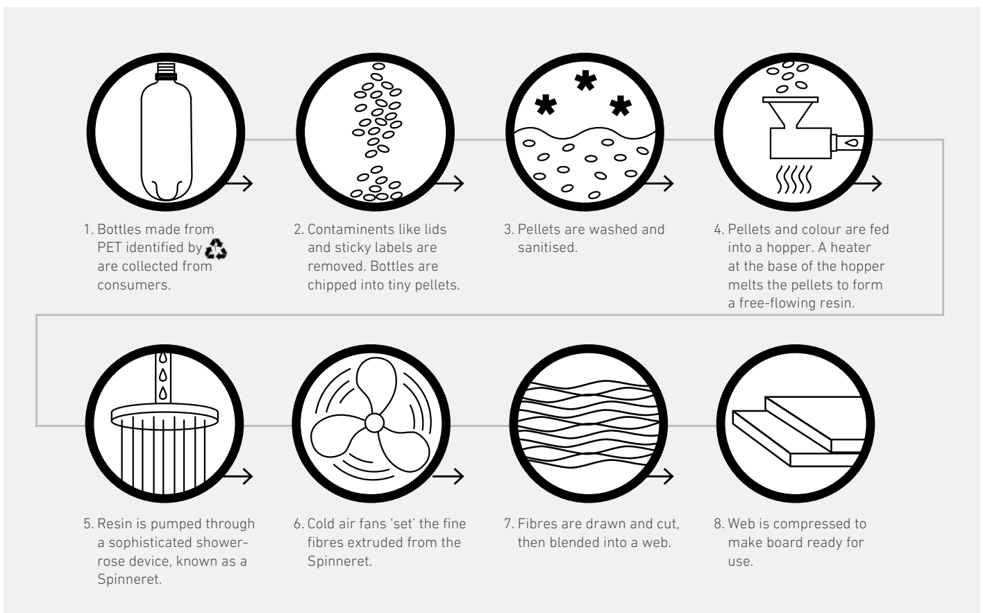
Figure 1: Manufacturing process of EchoPanel® and Mura™
