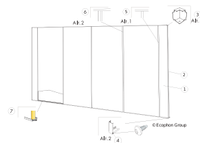
Installation diagram (M504) for Ecophon Akusto Wall A
