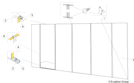
Installation diagram (M593) for Ecophon Akusto Wall A vertical installation with Connect Thinline profiles.
