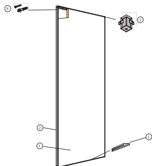
Installation diagram (M593) for Ecophon Akusto Wall A vertical installation with Connect Thinline profiles.
