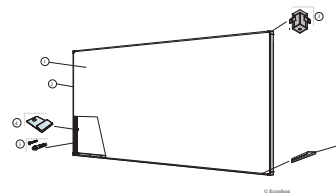
Installation diagram (M595) for Ecophon Akusto Wall A horizontal installation with Connect Thinline profiles.
