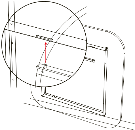
L-PROFILE: 50MM WALL DISTANCE With air gap & Quick-Release
