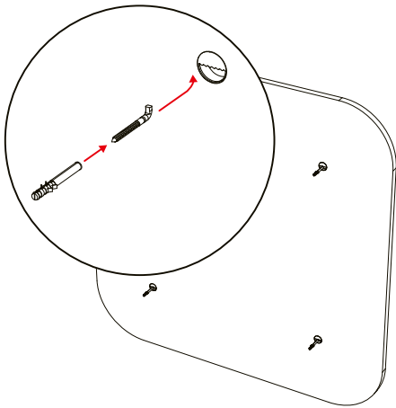
INLAY: 0-10MM WALL DISTANCE Direct mount & Quick-Release The INLAY System is only compatible with EchoBoard® 24mm
