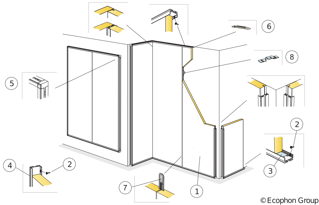
Installation diagram (M354) for Ecophon Akusto Wall C vertical installation
